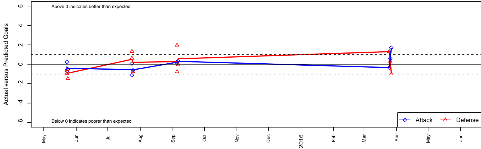
PSPL Academy 2001B Dots are actual minus expected GF (blue circles) and GA (red triangles). Blue line is smoothed change in attack strength. Red is smoothed change in defense strength.
